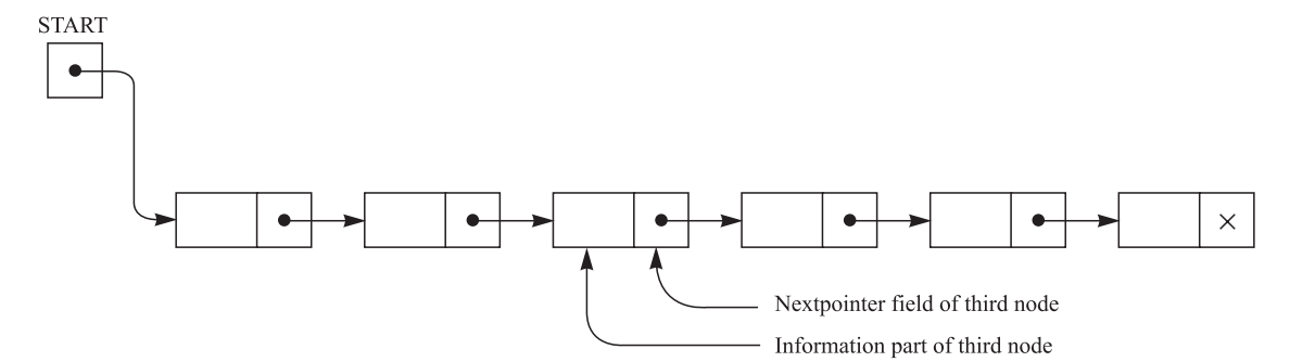
Fig. 8-1 Linked list with 6 nodes
